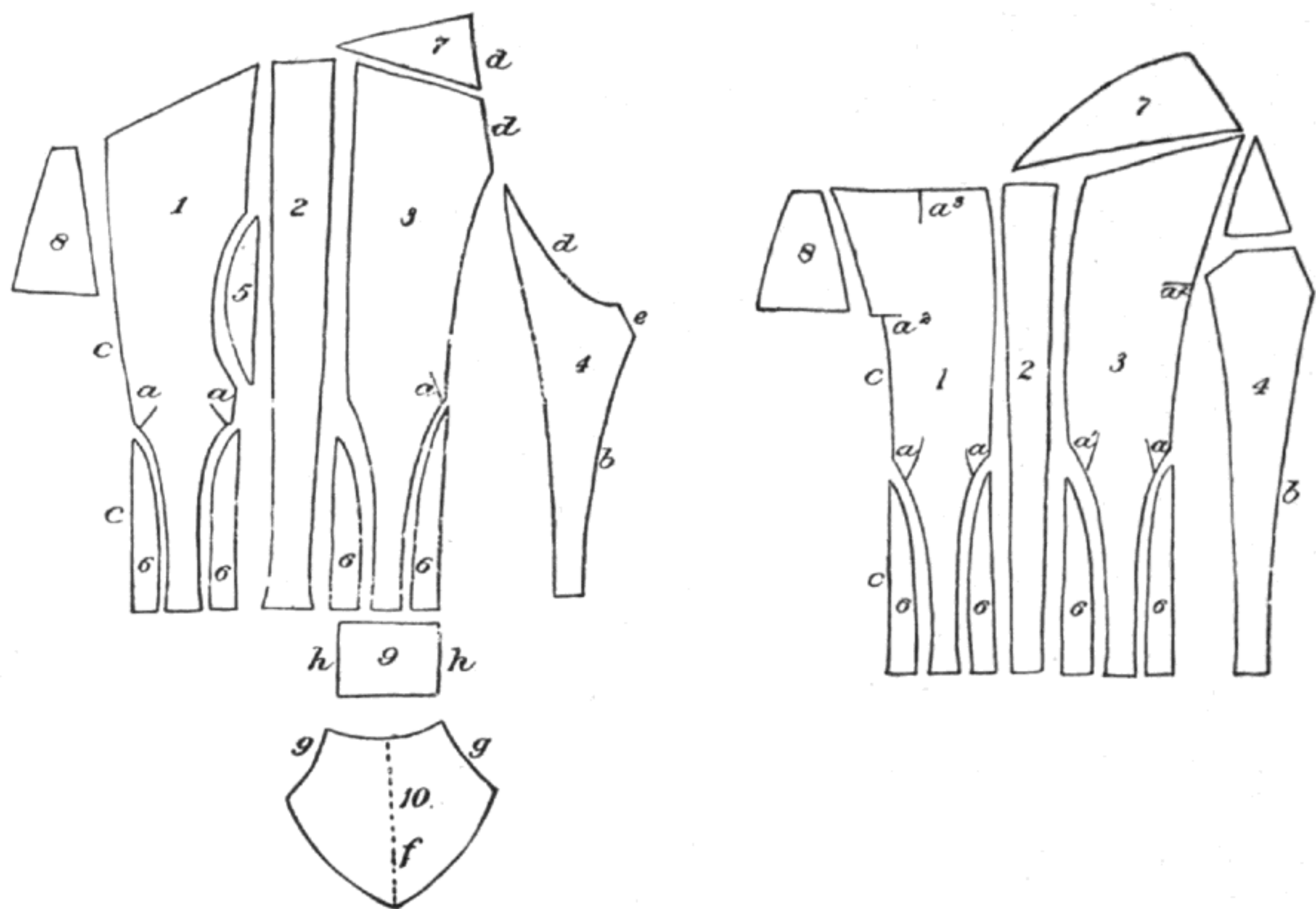
FIG. 73.—Patterns of woman's pantaloons.
